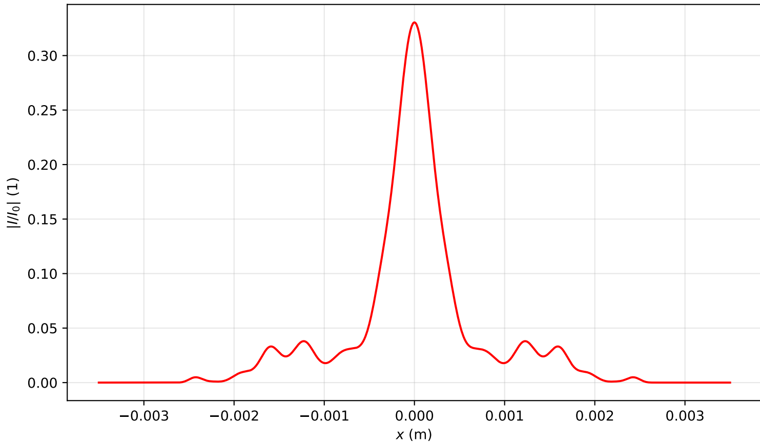
Intensity profile I(x, y = 0, z = 3.582)/I_0 , P_{in}=5.0P_{cr} , artificial time
